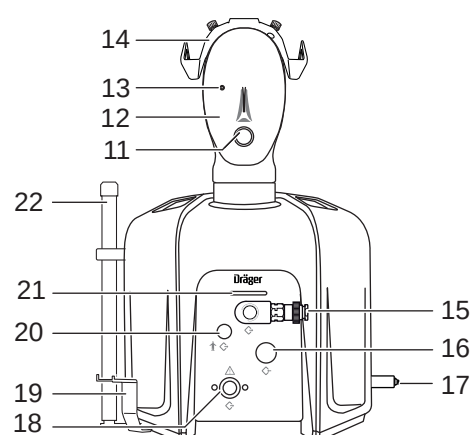
Dräger Quaestor 8000 (viewed from front)
