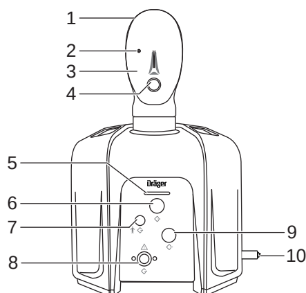
Dräger Quaestor 6000 (viewed from front)
