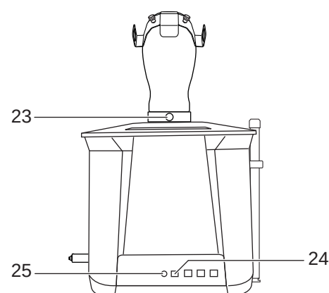
Both test units (viewed from rear)
