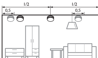
Fig. 1.5 Rooms with straight ceilings
