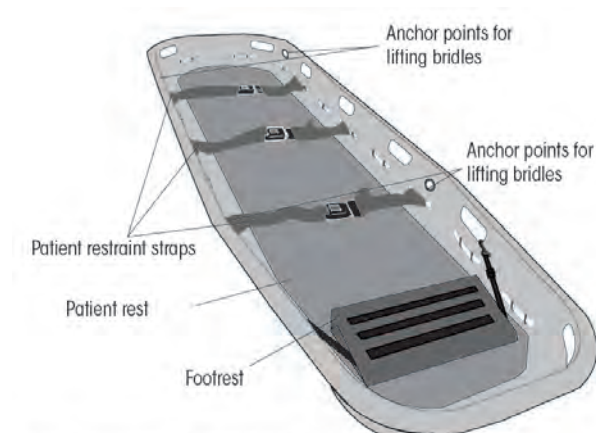
Image 1: Components of basket stretcher and anchor points
