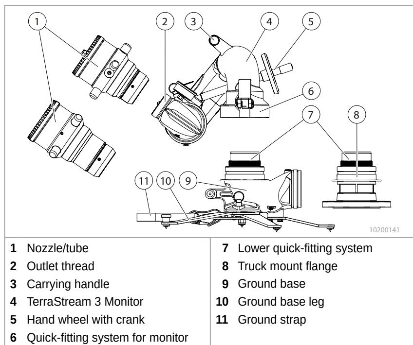
Fig. 1 Main components of the TerraStream 3 system
