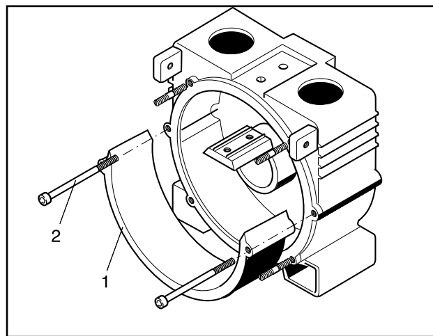
Abb. 21 Demontage Widerlager
