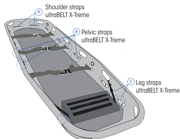
Image 7: Attaching the ultraBELT X-TREME strap system
