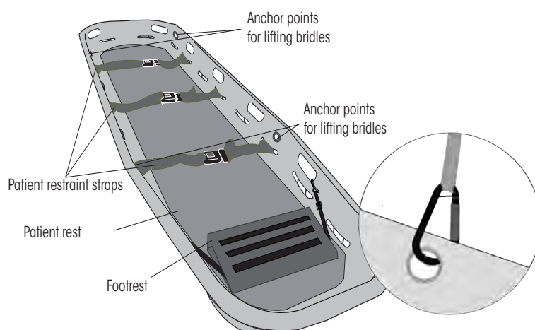
Image 1: Components of basket stretcher and anchor points
